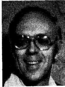
CHIP HENDRICKSON
